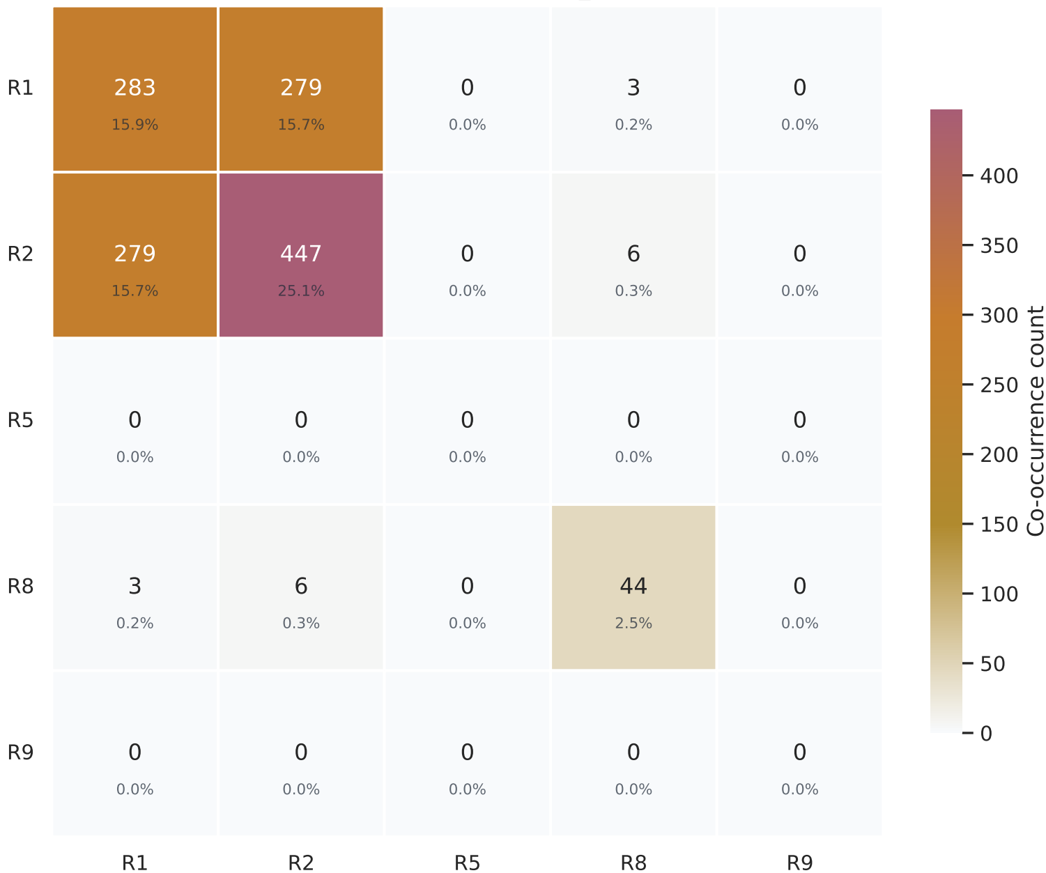
Tier 1 rule co-occurrence within dirty_4581 (n=1,779)
